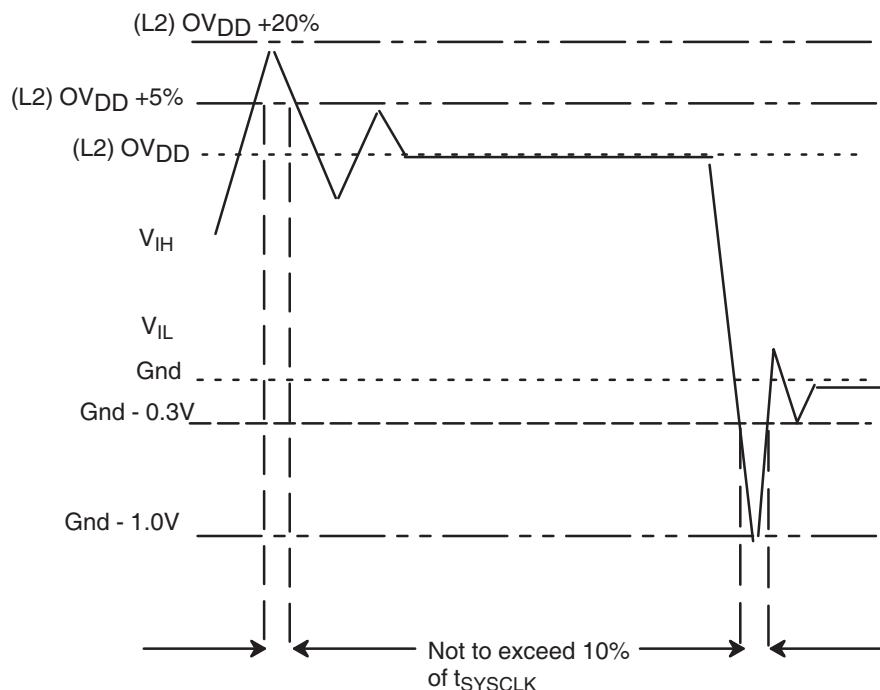
Figure 5-1. Overshoot/Undershoot Voltage
